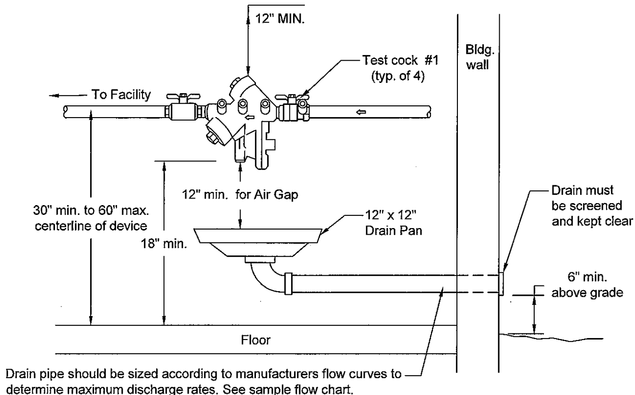
FRONT VIEW
